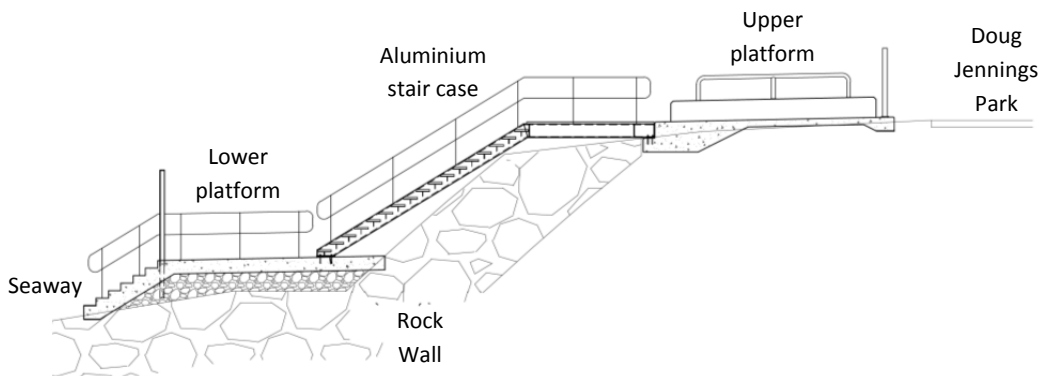
Figure 1. Typical Cross Section of Seaway South Emergency Access
